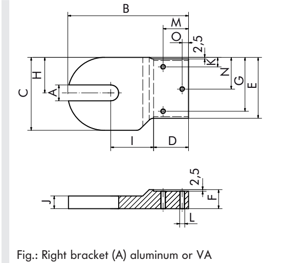
DM 0113, DM 0138 and DM 0165 dimensions
