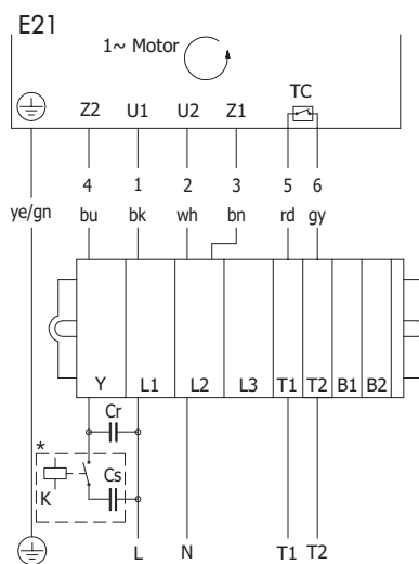
Fig.: 1-phase, 7-core cable
