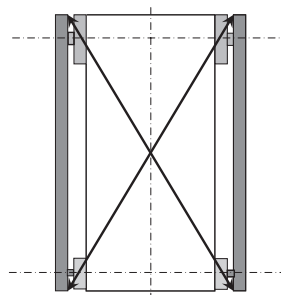
Fig.: Diagonal check
