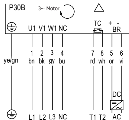
Fig.: With brake, 3-phase, 7+2 core cable, winding for 1 voltage, delta connection
