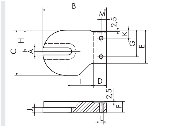
Fig.: Right bracket (A) aluminum or VA
